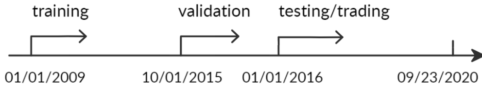
Figure 3: Data splitting.
