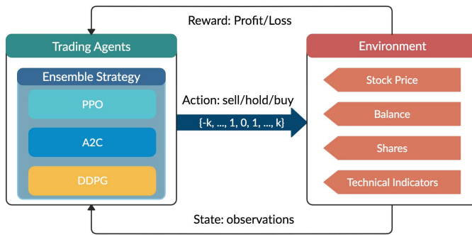
Figure 1: Overview of reinforcement learning-based stock trading strategy.
